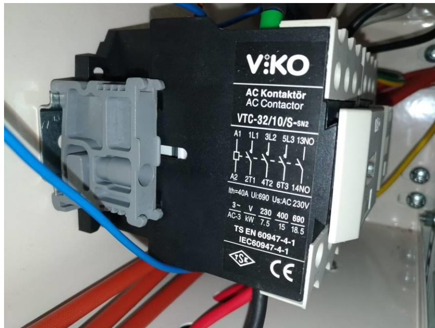
Image :3 ( Contactor )
